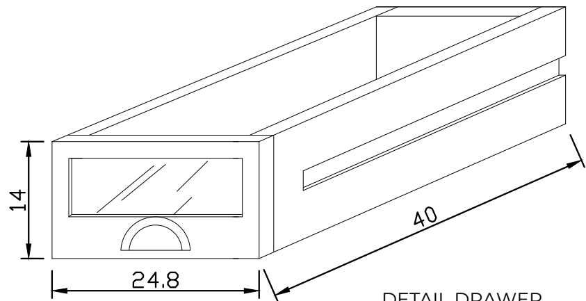
DETAIL DRAWER
