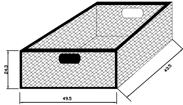
DETAIL BASKET
