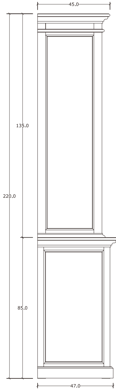
SIDE VIEW
