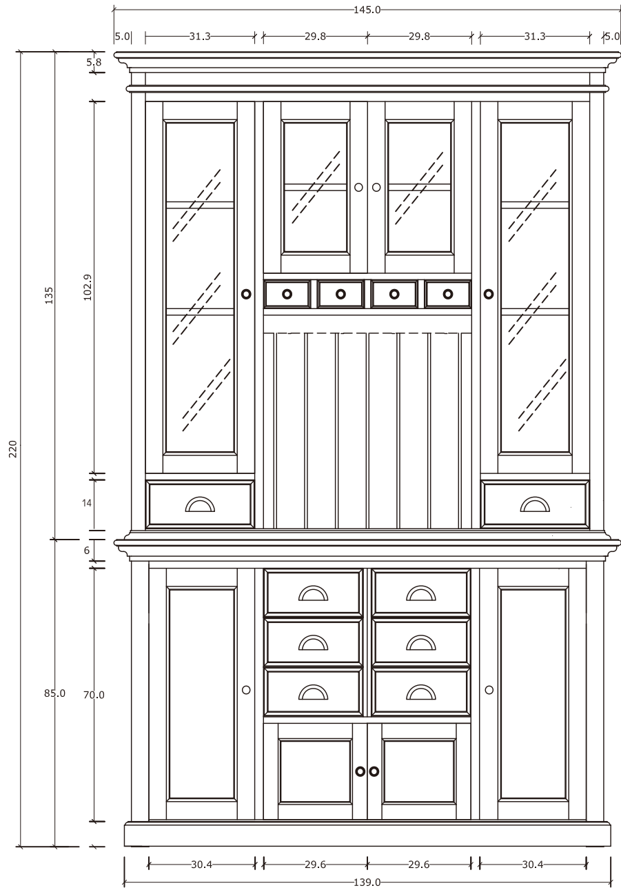
FRONT VIEW
