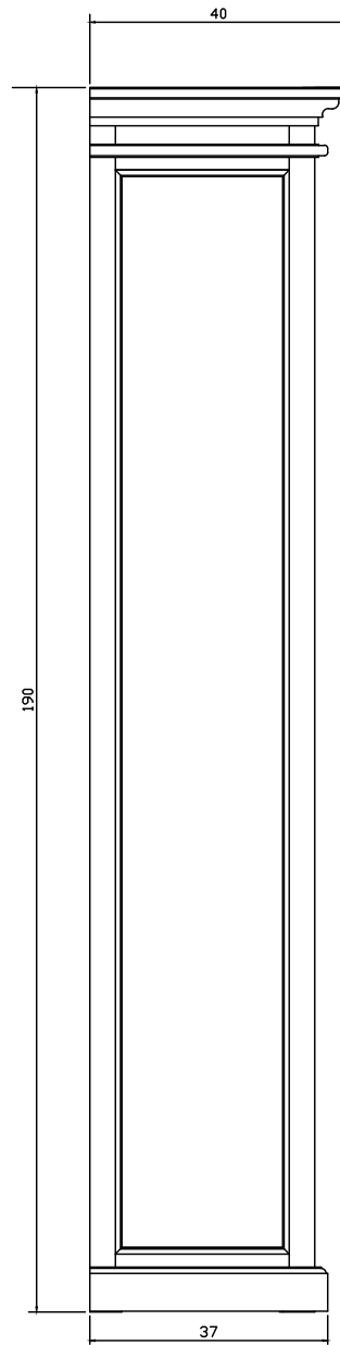
SIDE VIEW
