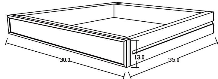
DRAWER DESIGN
