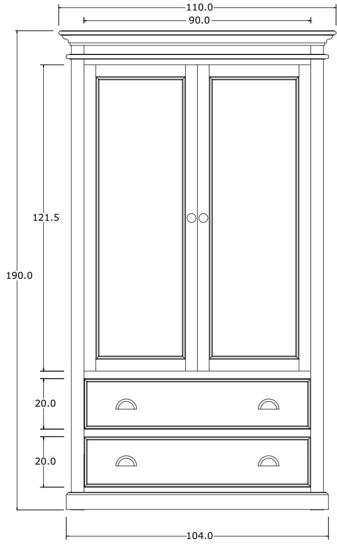
FRONT VIEW
